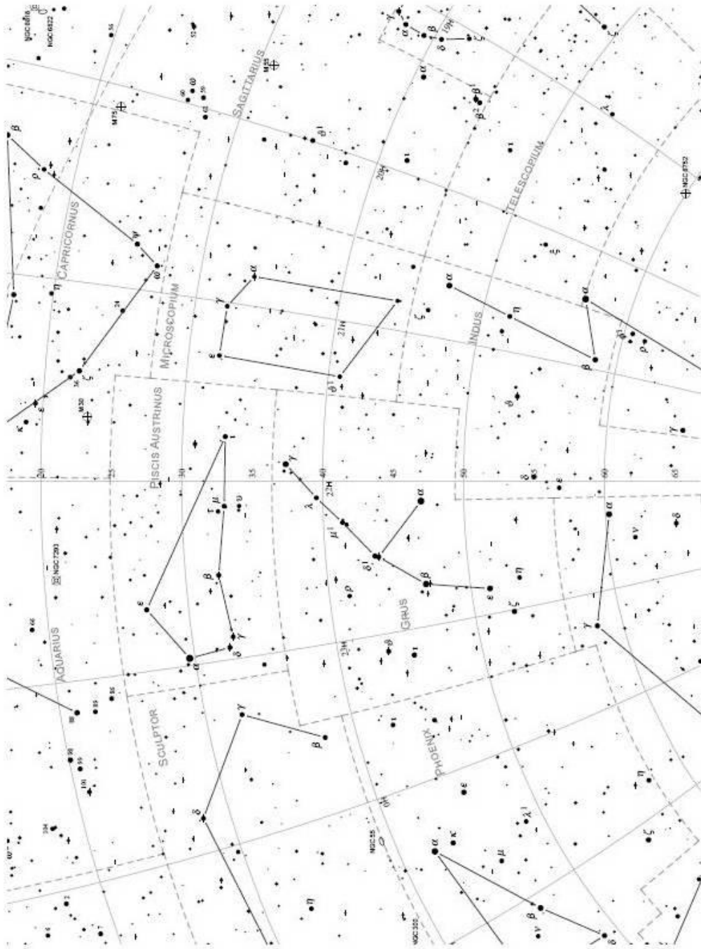
Chart 19: RA 20 h to 0 h , Declination -20° to -65° Mag-7 Star Atlas Project (version 2.0) Magnitude: 0.0 1.0 2.0 3.0 4.0 5.0 6.0 7.0 Copyright © 2007 Andrew L. Johnson
