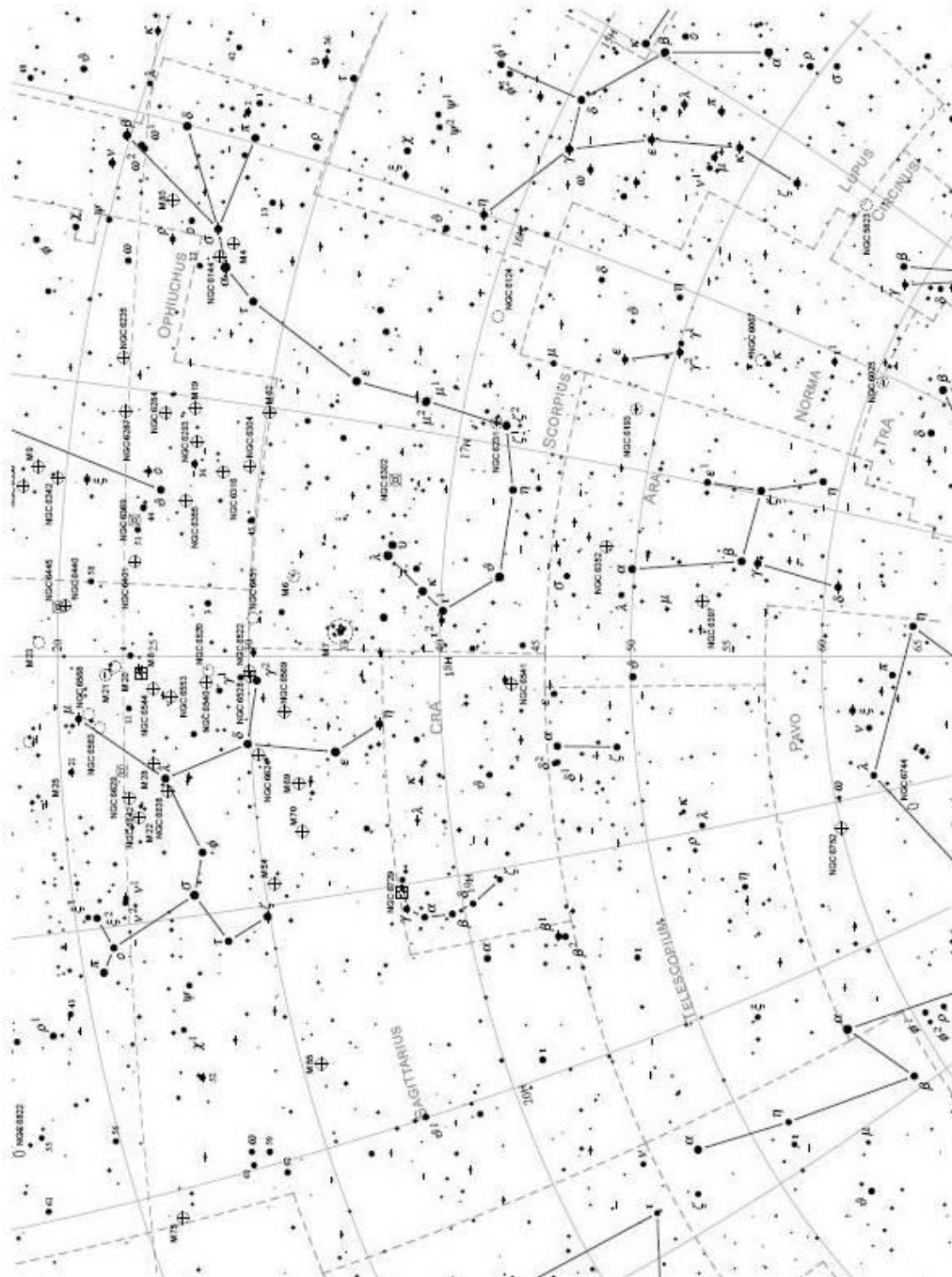
Chart 18: RA 16 h to 20 h , Declination -20° to -65° Mag-7 Star Atlas Project (version 2.0) Magnitude: 0.0 1.0 2.0 3.0 4.0 5.0 6.0 7.0 Copyright © 2007 Andrew L. Johnson
