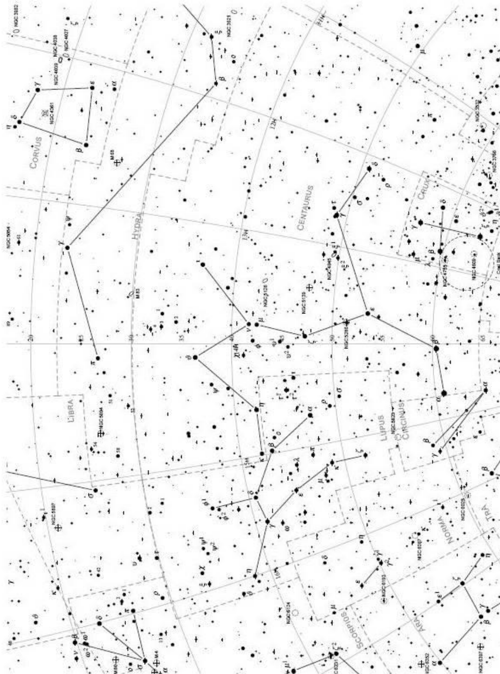
Chart 17: RA 12 h to 16 h , Declinations - 20° to - 65° Mag-7 Star Atlas Project (version 2.0) Magnitude: 0.0 1.0 2.0 3.0 4.0 5.0 6.0 7.0 Copyright © 2007 Andrew L. Johnson
